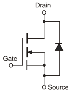
Equivalent Circuit
